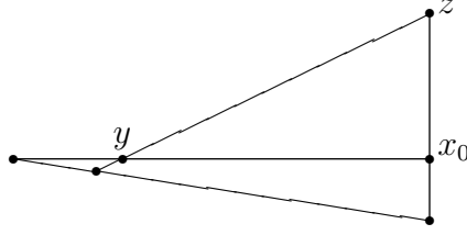
Figure 1.1: If the line segment from an interior point x_0 to y can be extended, then the line segment from any point z to y also can be extended
