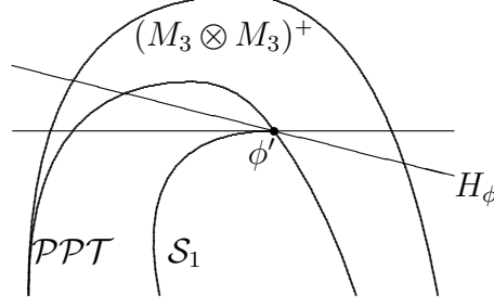
Figure 2.9: Entanglement W_\phi[(M_m \otimes M_n)^+, \mathcal{S}_1] detected by \phi is maximal, but PPT entanglement W_\phi[\mathcal{PPT}, \mathcal{S}_1] detected by \phi is not maximal.
