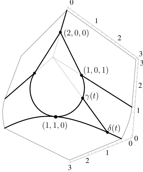
Figure 2.8: The surface bc = (1 - a)^2 consists of line segments.
