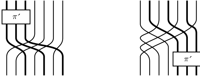
(a) The construction of element of \mathcal{S} (b) The construction of element of \mathcal{T}
